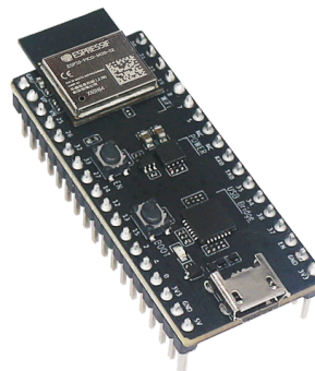
ESP32-PICO-DevKitM-2
