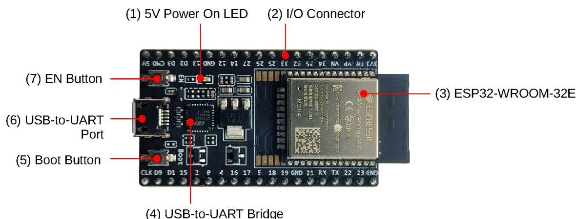
Fig. 1: ESP32-DevKitC V4 with ESP32-WROOM-32E module soldered
