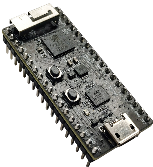
ESP32-PICO-KIT-1
