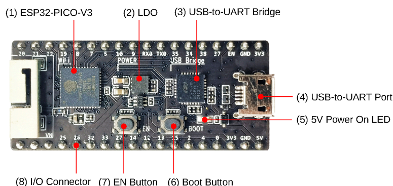
Fig. 2: ESP32-PICO-KIT-1 board layout - front (click to enlarge)
